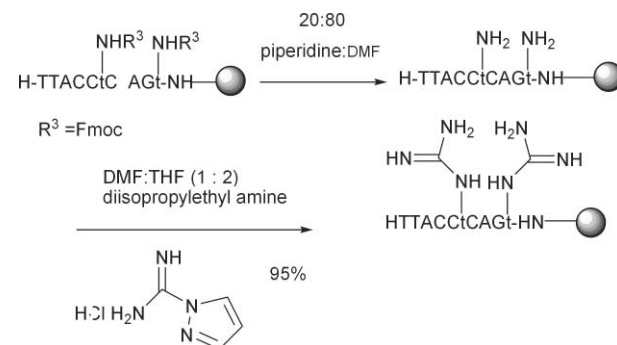
Scheme 3 Post-synthetic conversion of amino to guanidino functionality
